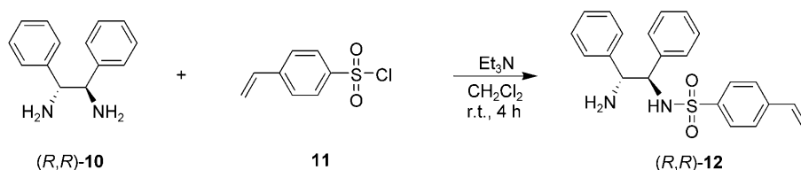
Scheme 1. Synthesis of chiral 1,2-diamine monosulfonamide monomer (R,R) -12.
