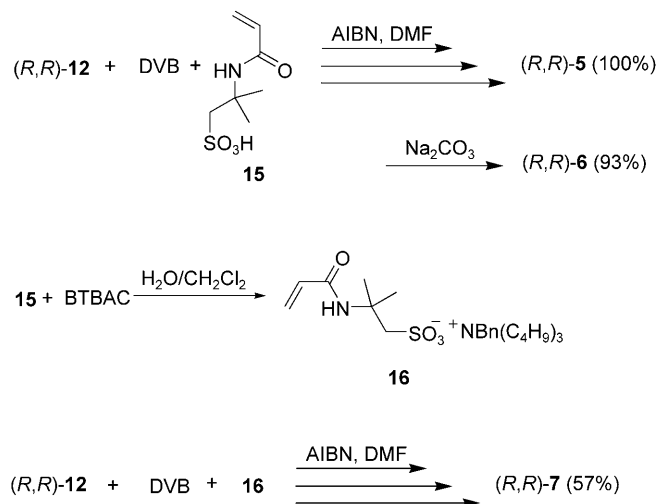
Scheme 4. Preparation of sulfonated polymer-supported chiral 1,2-diamine monosulfonamides ( R,R )- 5–7 .
