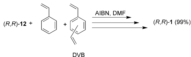
Scheme 2. Preparation of cross-linked polystyrene-supported chiral 1,2-diamine monosulfonamide (R,R) -1.
