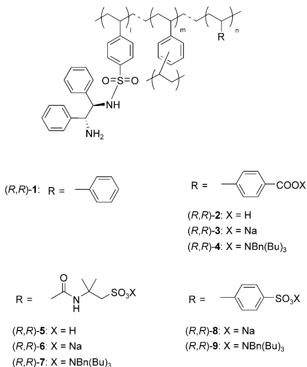
Figure 1. Polymer-supported chiral 1,2-diamine monosulfonamides.
