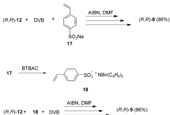
Scheme 5. Preparation of aromatic sulfonated polymer-supported chiral 1,2-diamine monosulfonamides ( R,R )- 8 and 9 .
